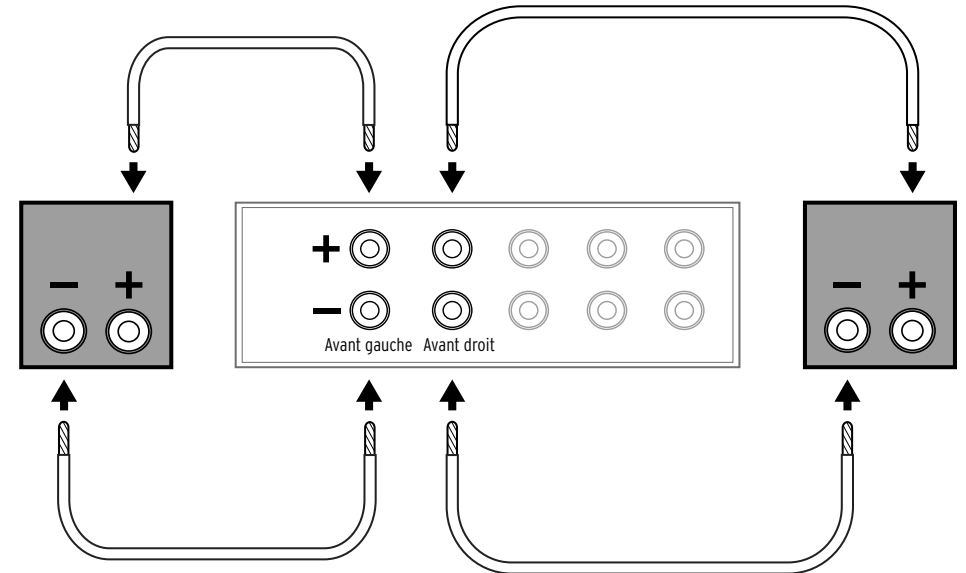
FIGURE 3 BRANCHEMENTS STANDARD
