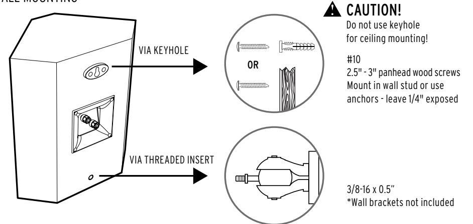
FIGURE 4 WALL MOUNTING
